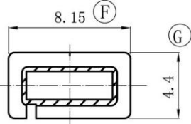
B-B SECTION
