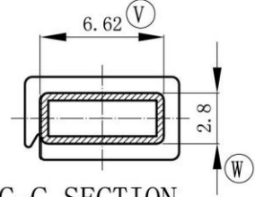
C-C SECTION
